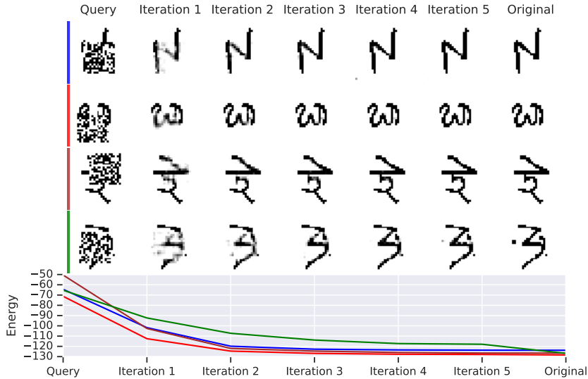
Figure 2: Visualization of gradient descent iterations during retrieval of Omniglot characters (largest model). 4 random images are shown from the batch of 64.
