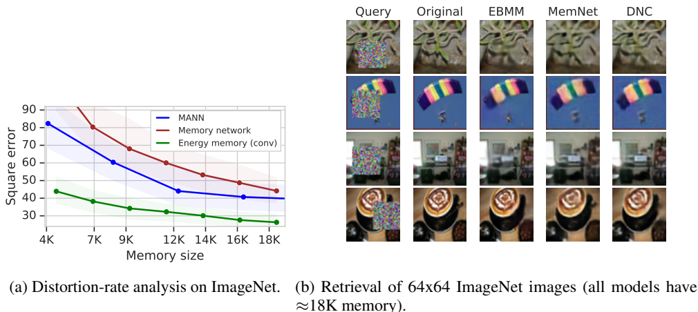
Figure 5: ImageNet results.
